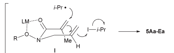
Scheme 3 Reaction of substrates 4A–E .
