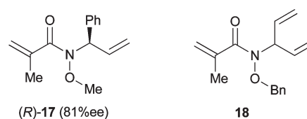
Fig. 5 Substrates ( R )-17 and 18.
