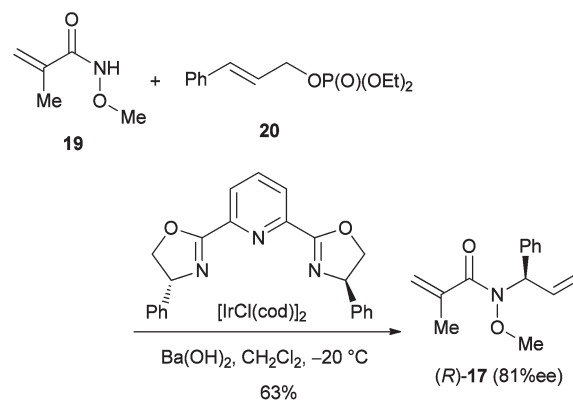
Scheme 8 Preparation of substrate ( R )-17.
