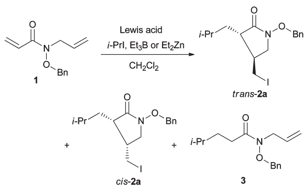
Scheme 1 Reaction of substrate 1 having an acryloyl moiety.
