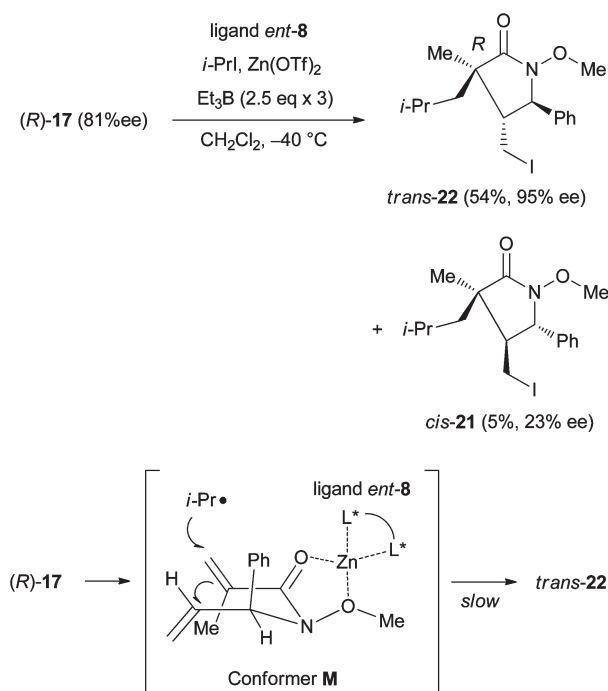
Scheme 10 Reaction using ligand ent - 8 .
